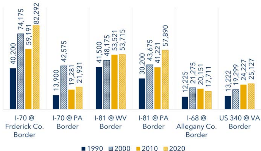
Chart 7-5: AADT Count at Major County Entrances/Exits
