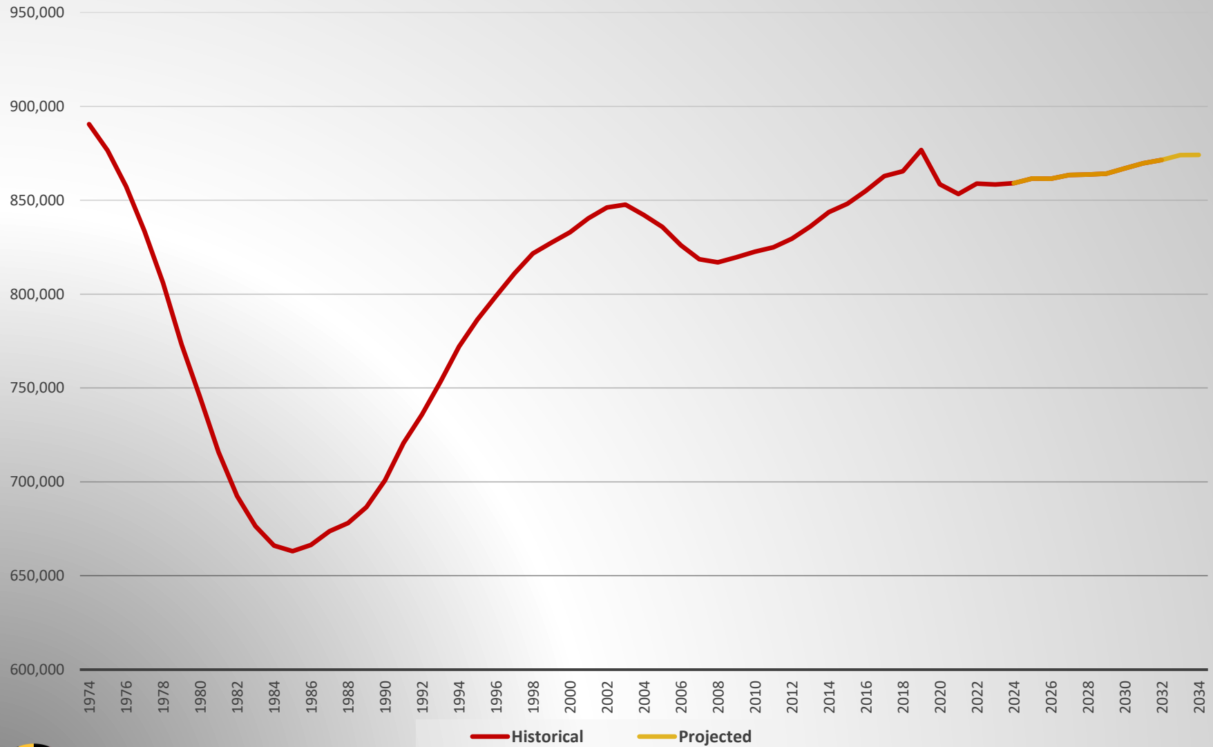
Chart 6. Total Public School Enrollment in Maryland, Historical and Projected, 1974 - 2034 *
