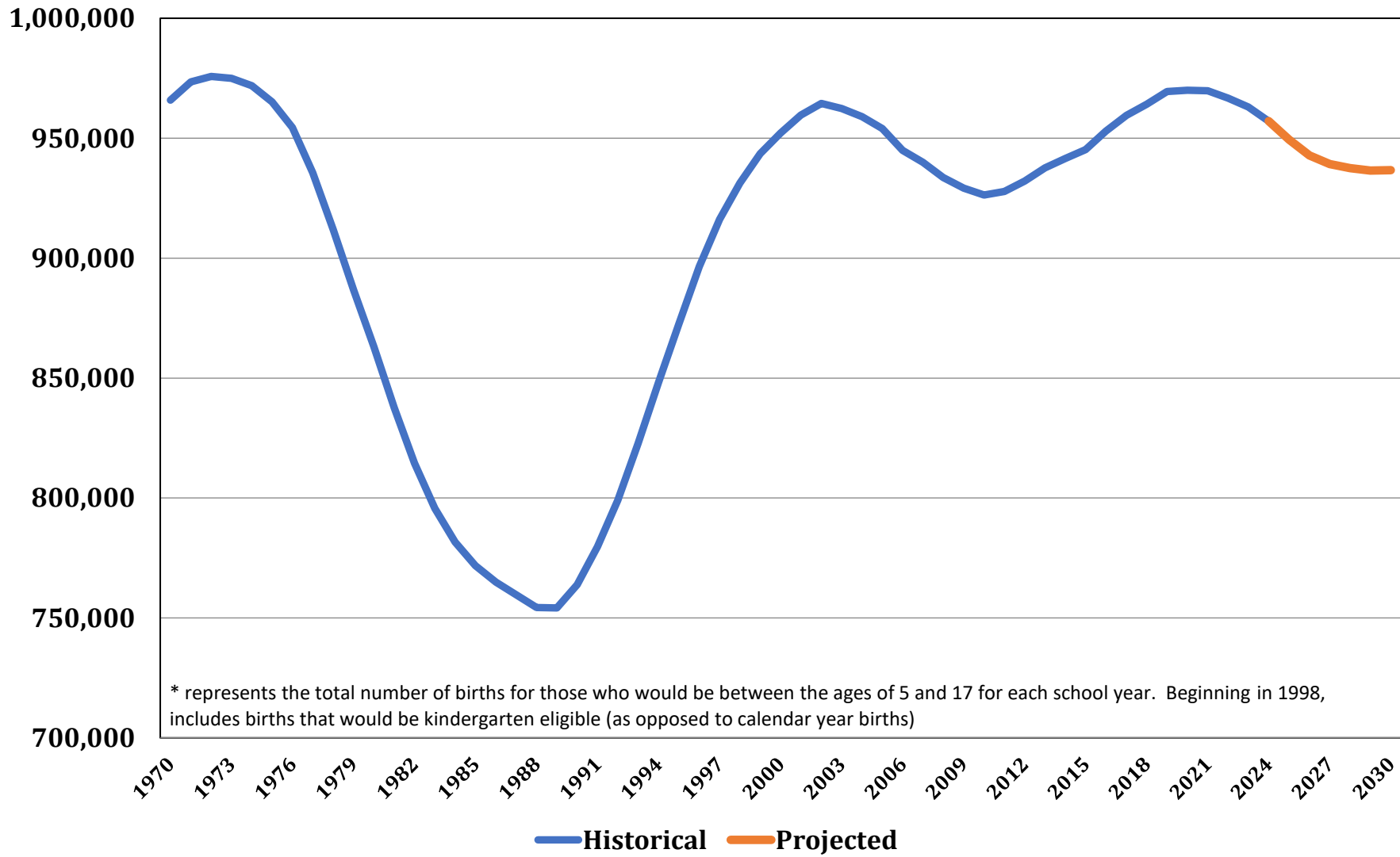
Chart 8. Cumulative Births by School Year in Maryland Historical & Projected, 1970 - 2030 *
